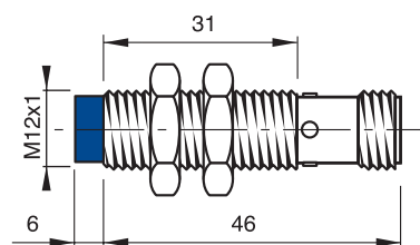
CONFIGURATION WITH CONNECTOR M12
